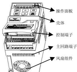
II类外观 适用机型 DL100-2S0007(B)~DL100-2S0015(B) DL100-4T0007(B)~DL100-4T0015(B)
